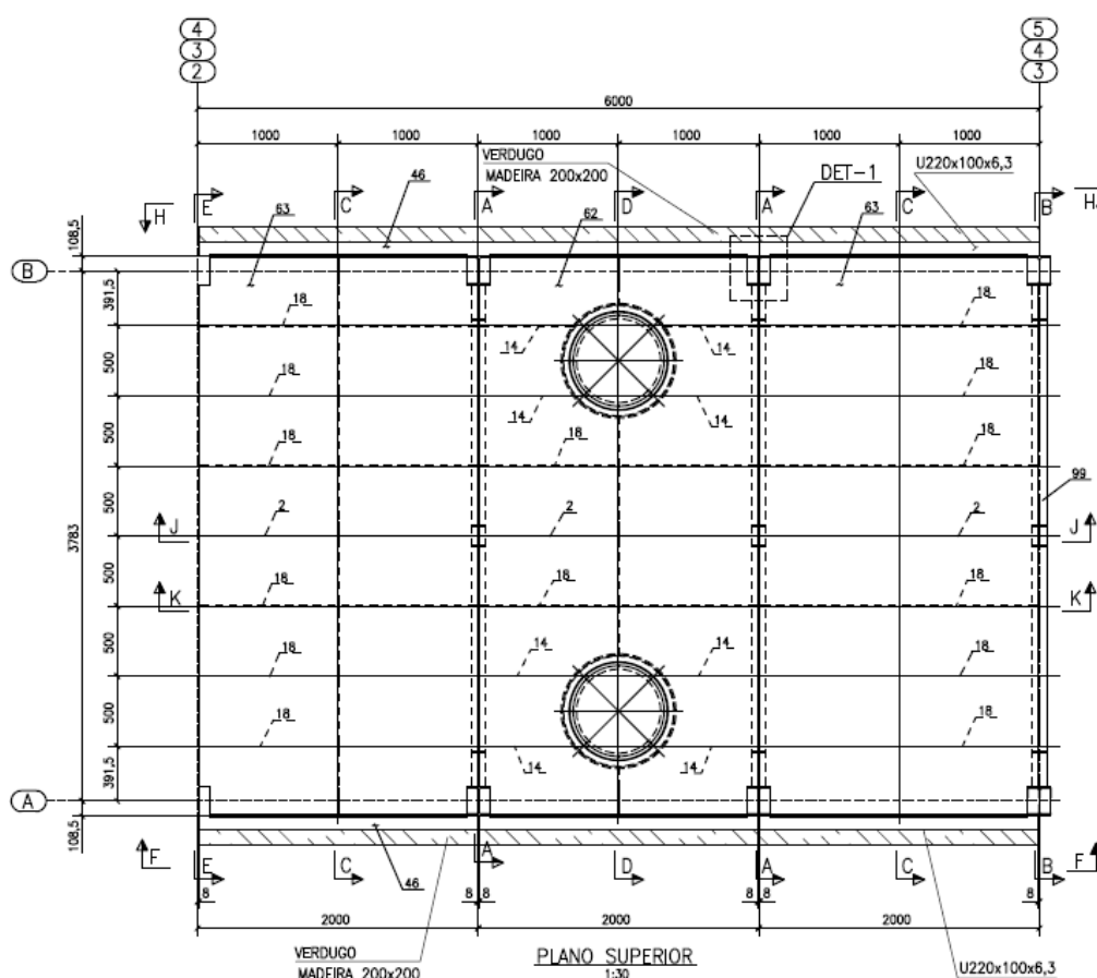
FIGURA 11 – FLUTUANTES – PLANTA SUPERIOR
